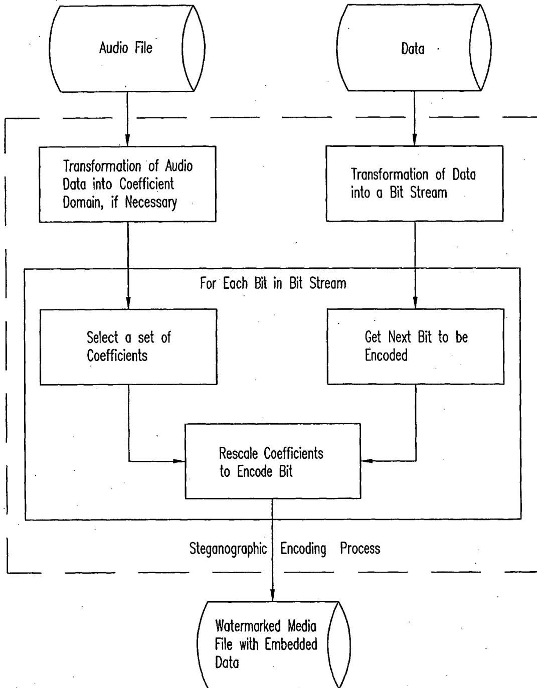
Encoding Data in an Audio File
